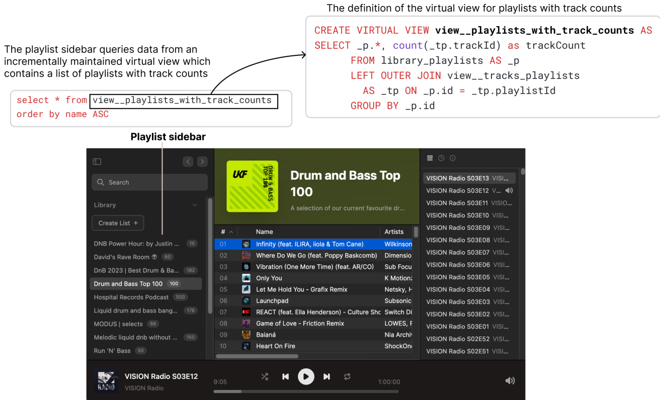
Figure 4: Examples of a SQL query and view definition used in the Overtone music manager.
