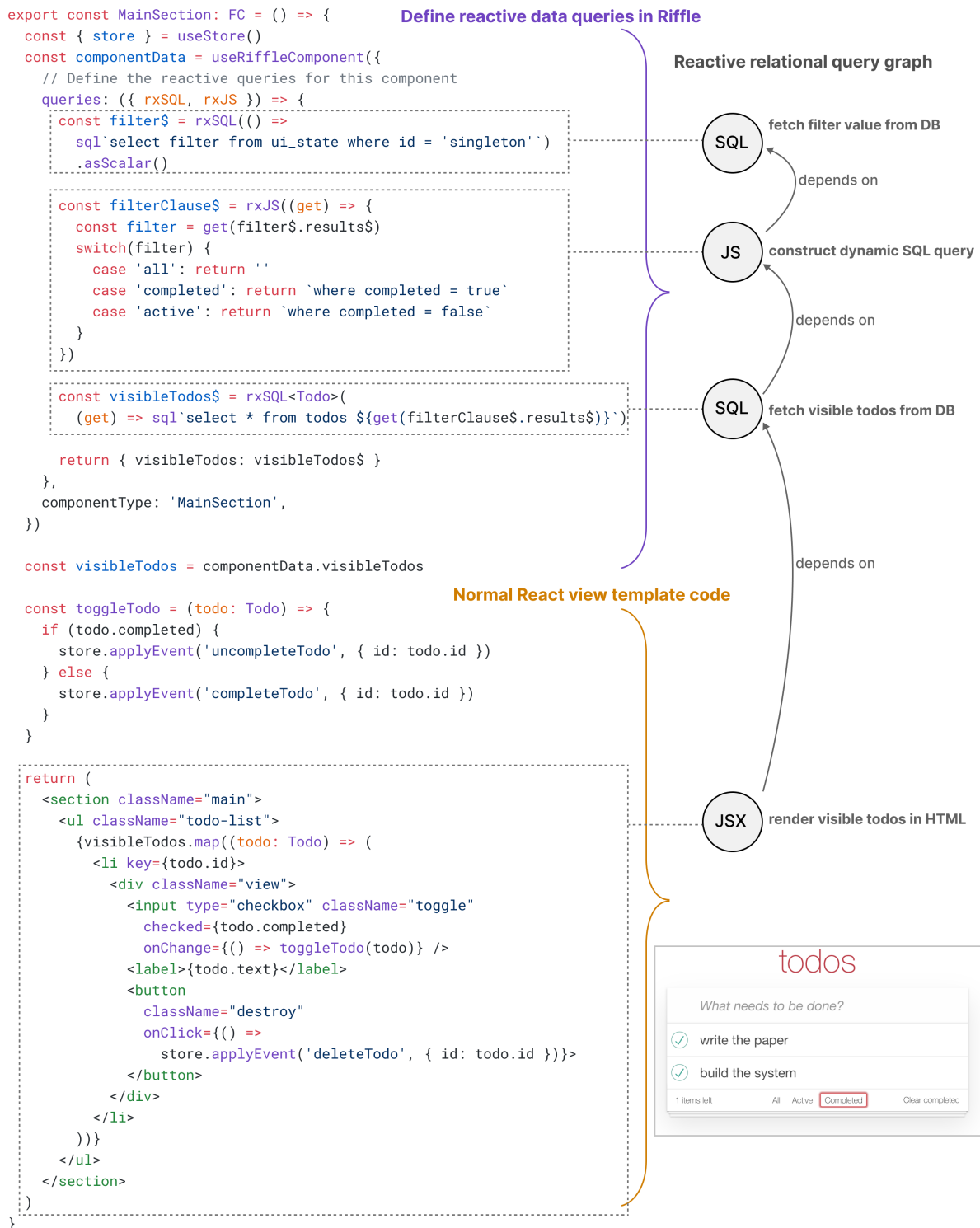
Figure 3: TodoMVC includes a simple example of a dynamic SQL query. The currently active filter setting is queried from a table using a SQL query. A JavaScript query then turns that value into a filter clause in a SQL string, which in turn queries the todos table to produce the final filtered data for the view.
