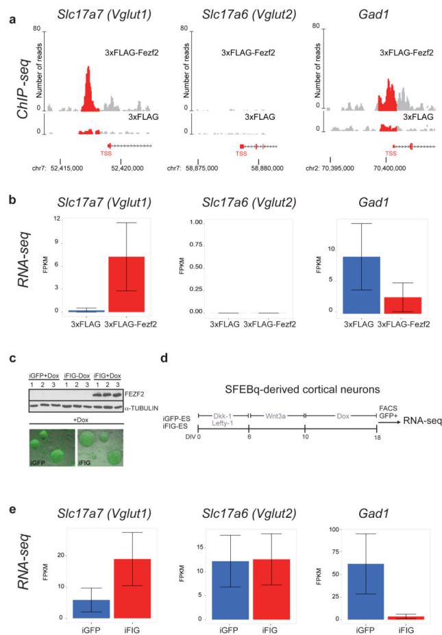
Figure 4. Fezf2 promotes glutamatergic and inhibits GABAergic neurotransmitter pathways. (a) ChIP-seq trace shows that 3xFlag- Fezf2 binds specifically to the promoters of Vglut1 ( Slc17a7 ) and Gad1 but not Vglut2 ( Slc17a6 ). (b) RNA-seq analysis shows the effect of 3xFlag- Fezf2 overexpression on these three genes in neural stem cells in vitro . (c) Inducible expression of single-copy Fezf2-IRES-GFP is shown by immunoblotting and fluorescence microscopy. Uncropped original immunoblots are shown in Supplementary Figure 10. (d) Schematic representation of directed differentiation protocol used to instruct embryonic stem cell (ES) differentiation into mixed populations of cortical neurons 23 . (e) RNA-seq analysis showing the effect of Fezf2 expression on Vglut1 , Vglut2 and Gad1 in ES-derived neurons. Clones used for RNA-seq were from the differentiation of n = 2 independently generated iGFP and n = 2 iFIG lines. The error bars represent 95% confidence intervals for the Cuffdiff2 model expression estimate as defined in Methods and described in Trapnell et al., 2013.
